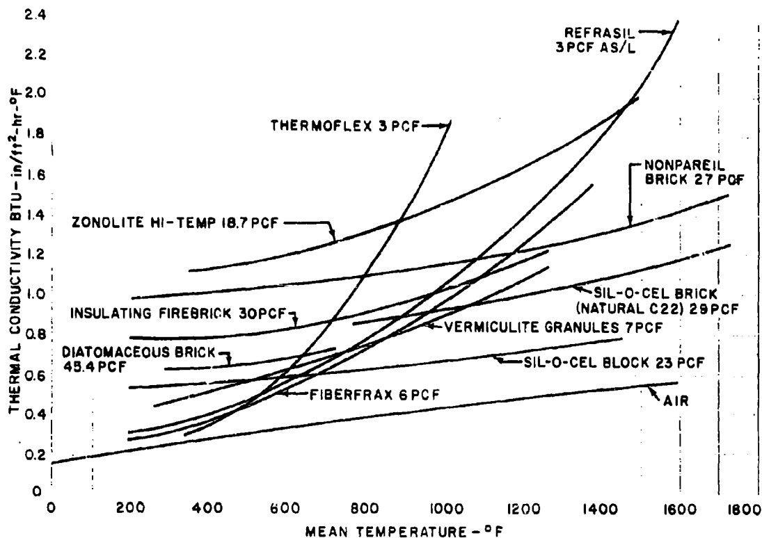
Figure 33. Thermal Conductivities of Insulators
