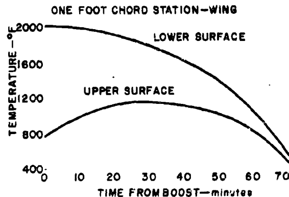
Figure 18. Equilibrium Temperature Time History
