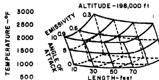
Figure 21. Equilibrium Temperature at Mach 20 for Turbulent Flow
