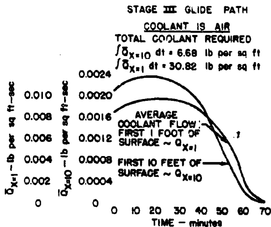
Figure 22. Average Coolant Flow vs Time for Transpiration Cooling of Wing Lower Surface to 1600°R
