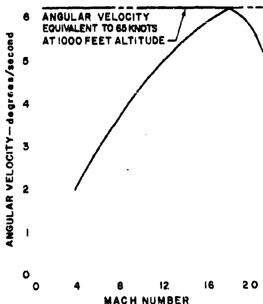
Figure 5. Equivalent Terrain Speed During Cruise of MX-2276
