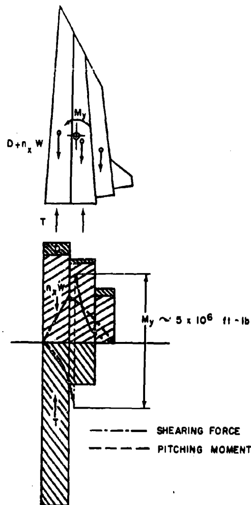
Figure 31. Typical Axial Acceleration Forces and Moments
