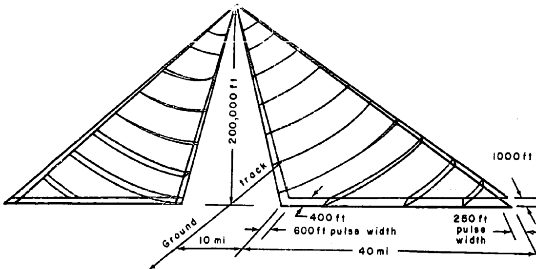
Figure 50c. Proposed Simultaneous-Lobing Radar: Ground Coverage
