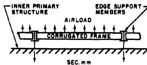
Figure 39. Structural Configuration Principles
