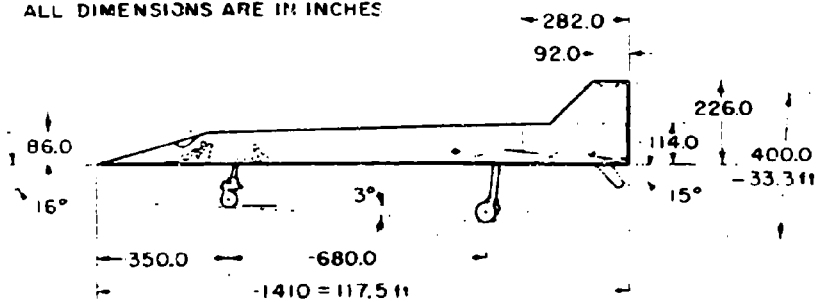
Figure 2. Initial Configuration of MX-2276 Stage I
