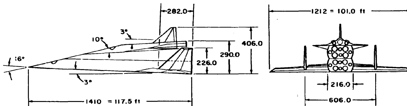
Figure 1. Initial Configuration of MX-2276
