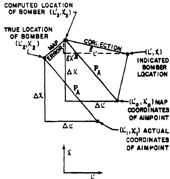
Figure 48. Position Correction of Navigation System
