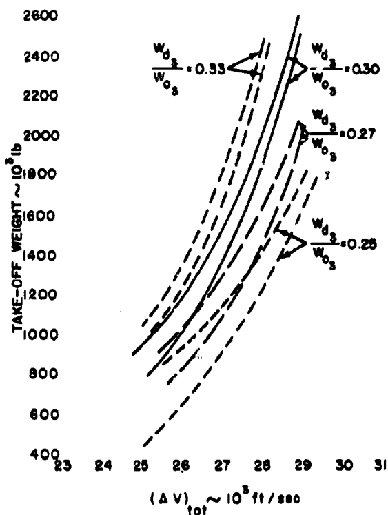
Figure 61. Take-Off Weight as a Function of Cut-Off Velocity
