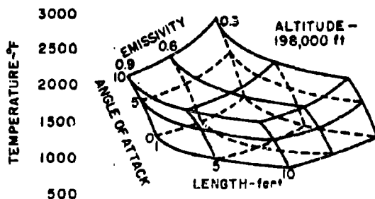
Figure 20. Equilibrium Temperature at Mach 20 for Laminar Flow
