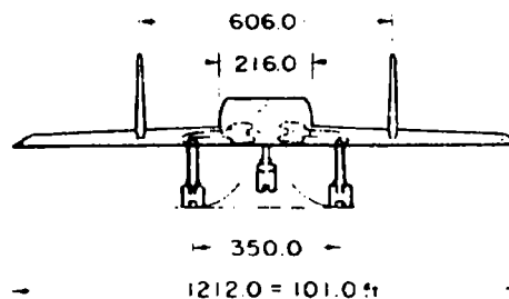
Figure 2. Initial Configuration of MX-2276 Stage I
