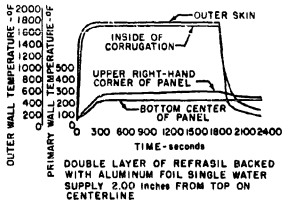
Figure 42. Thermal Cooling Test: Double Layer Refrasil
